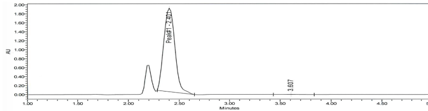
HPLC-MS Chromatogram
