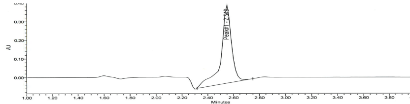
HPLC-MS Chromatogram
