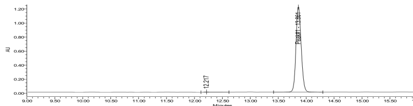
HPLC-UV Chromatogram
