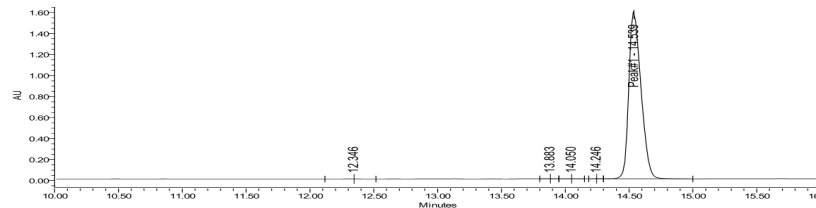
HPLC-UV Chromatogram
