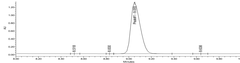
HPLC-UV Chromatogram
